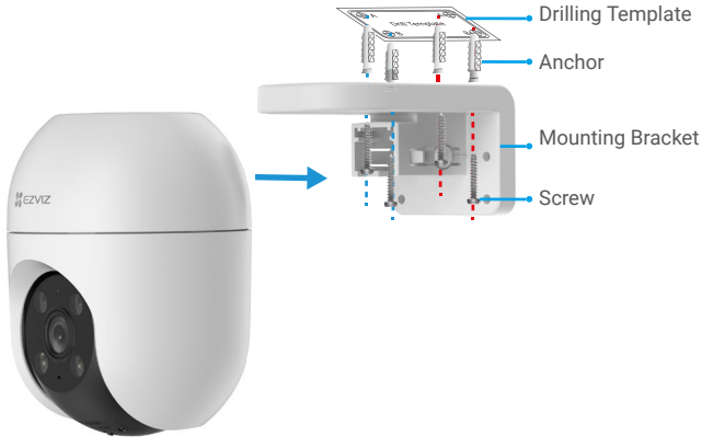
Fig. 1 Ceiling Mount
