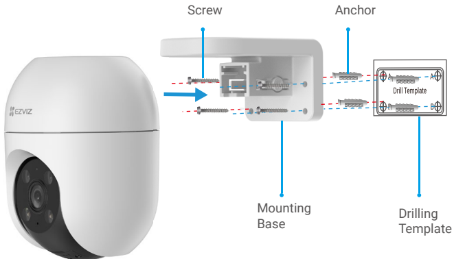
Fig. 2 Wall Mount
